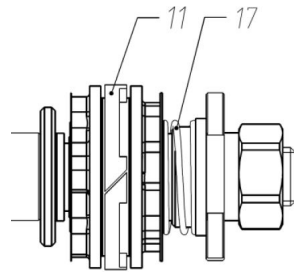
Compression rod
